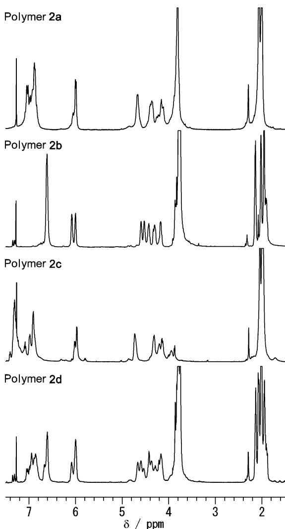
Fig. 3 ^1\text{H-NMR} spectra of acetylated \beta\text{-O-4} type artificial lignin polymers 2a–2d in \text{CDCl}_3 .
