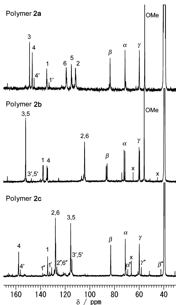
Fig. 1 ^{13}\text{C} -NMR spectra of \beta - O -4 type artificial lignin polymers 2a–2c in \text{DMSO-}d_6 . 1', 3', 4', 5': phenolic end units; 1'', 2'', 6'', \alpha' , \beta' , \gamma' : non-phenolic end units; x: solvents.
